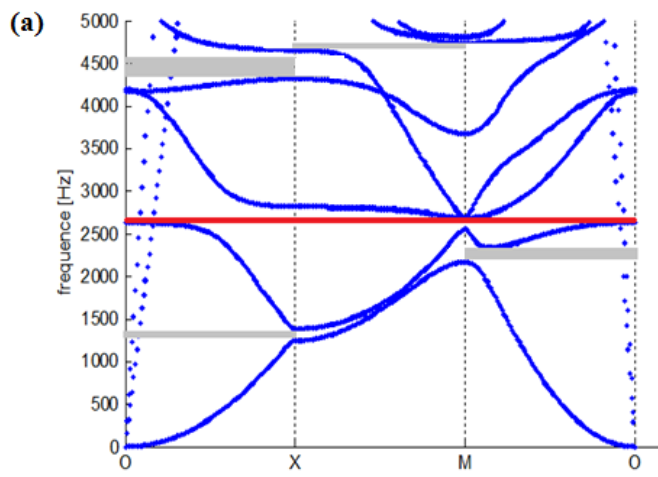
Figure 1 : (a) band diagram of a periodic composite plate with rubber inclusions, (b) unit cell with inclusion
